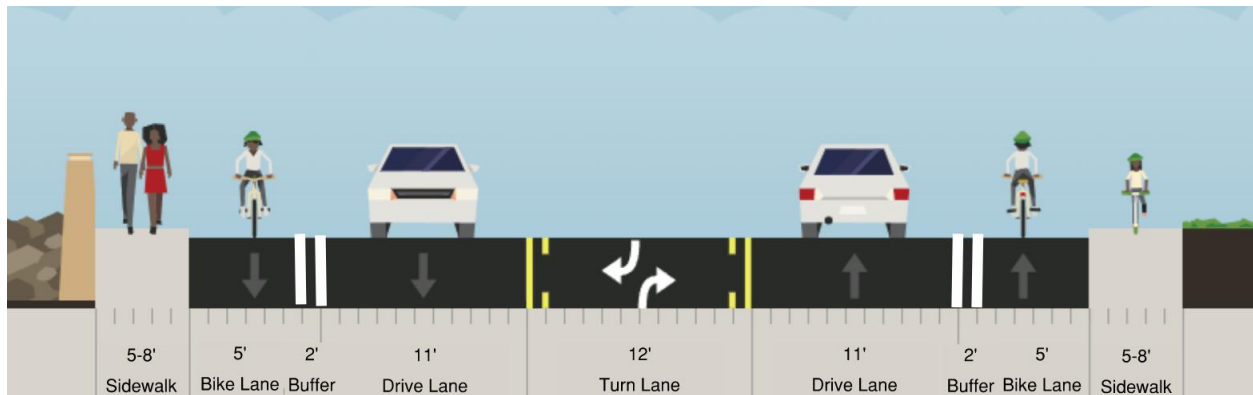
Figure 11. Recommended Typical Cross Section from Jerry's Flat Road to south of Harbor Way (Facing North)
