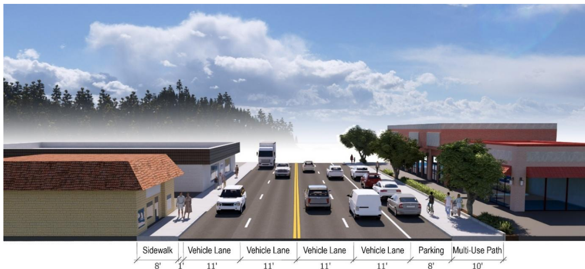
Figure E-1. Preliminary Most Promising Alternative A.4 4-Lane Section Rendering (Facing South)
