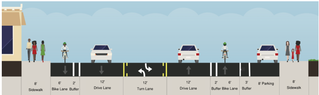
Figure 12. Recommended Typical Cross Section from Harbor Way to Moore Street (Facing North)
