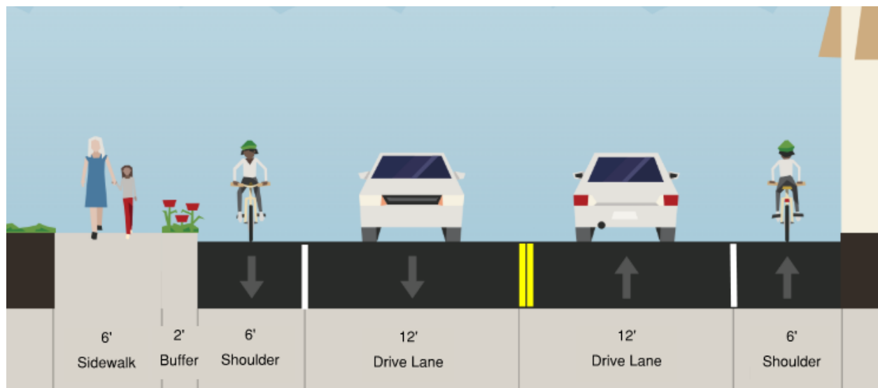
Figure 14. Recommended Typical Cross Section from Kerber Drive to Shirley Lane (Facing North)
