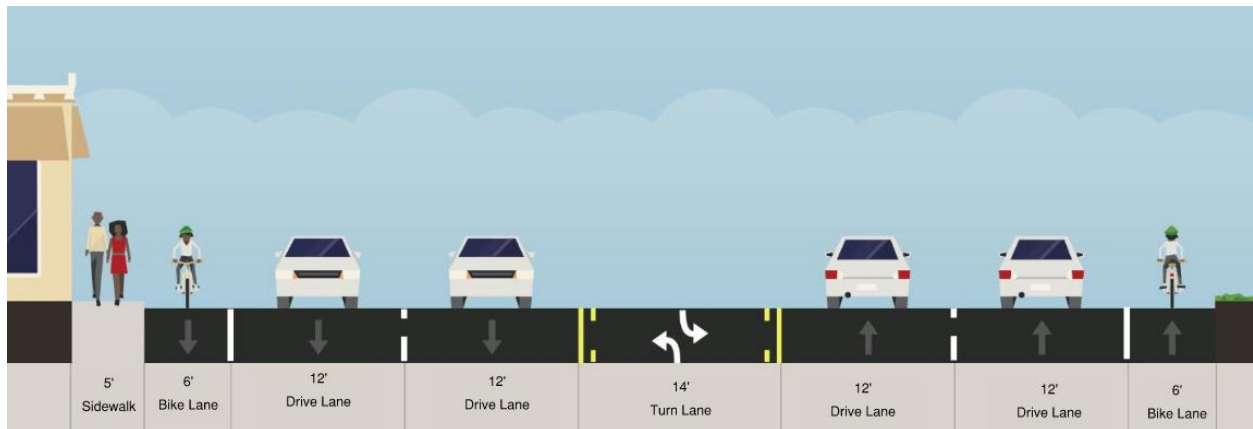
Figure 10. Existing Typical Cross Section from Harbor Way to Moore Street (Facing North)
